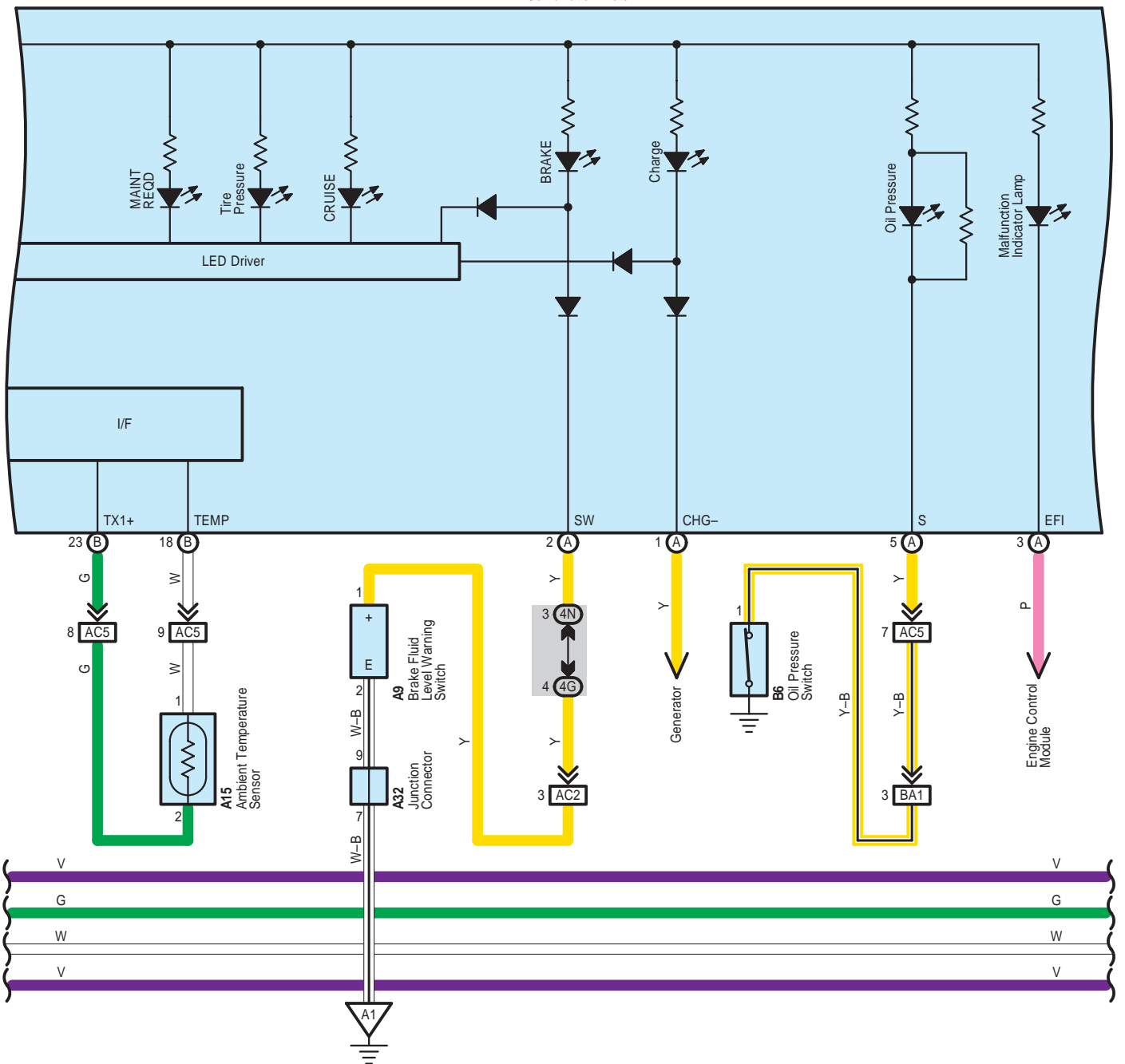
C36(A), C37(B) Combination Meter
